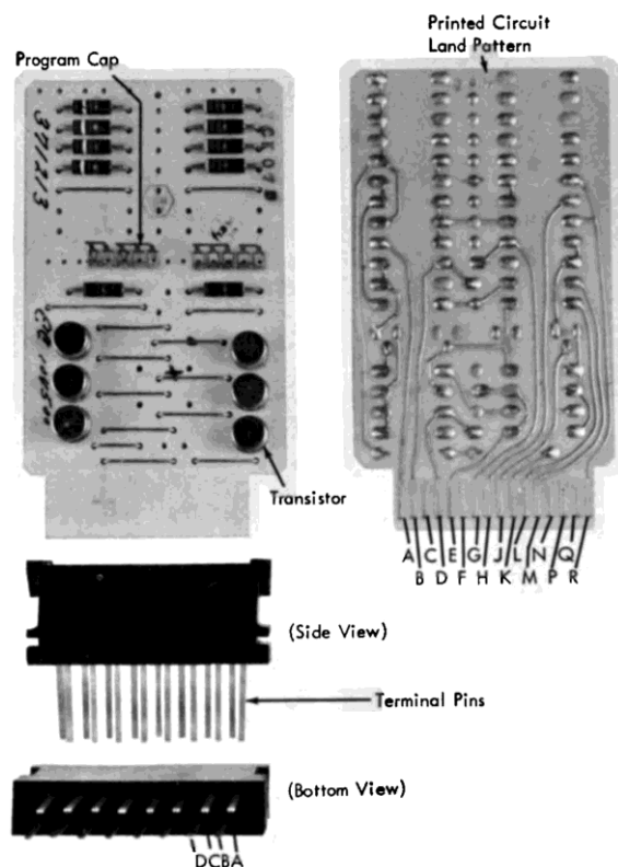
Figure 26. SMS Printed Wiring Cards Single Card and Socket
